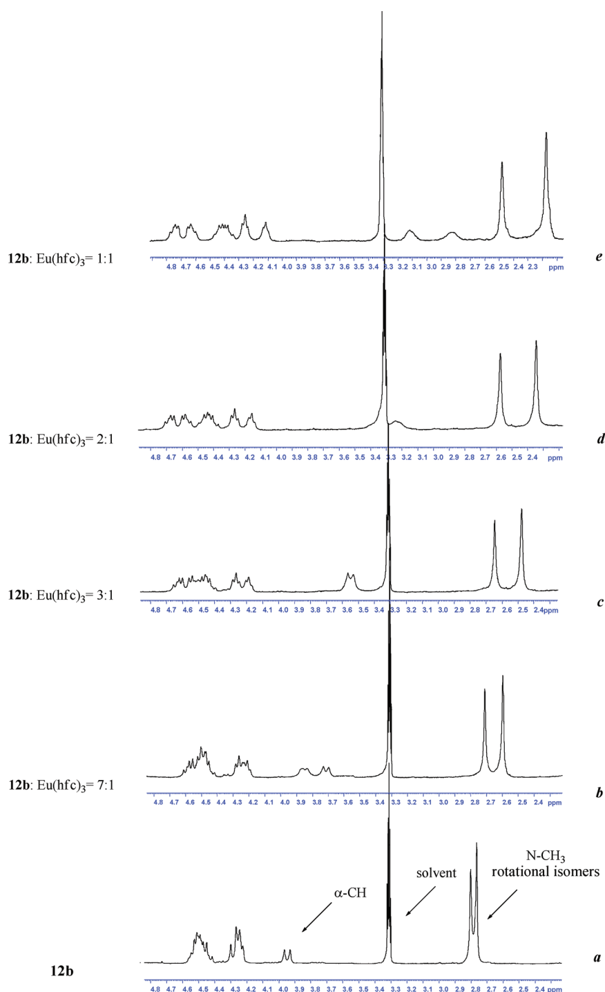
FIGURE 1. (a) The 300 MHz ^1\text{H} NMR spectrum of N -Fmoc- N -methyl-L-valine ( 12b ) in \text{CD}_3\text{OD} . (b–e) Spectra of various mixtures of 12b with the chiral shift reagent \text{Eu}(\text{hfc})_3 .
